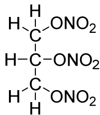
Figure 1. Structure of nitroglycerin.
