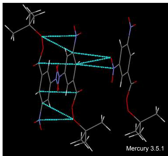
Figure 33. tert -Butyl peroxy ester group-aromatic ring and nitro group-aromatic ring interactions (blue) of 22 .
