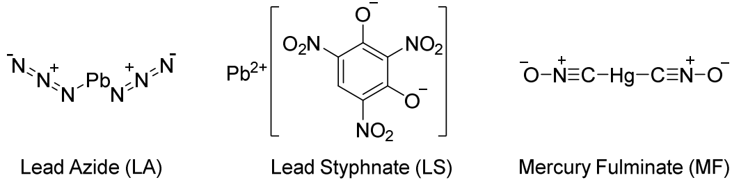
Figure 2. Common primary explosives.
