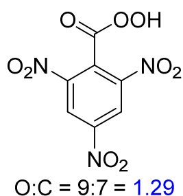
Figure 72. 2,4,6-Trinitrobenzoperoxoic acid ( 53 ).
