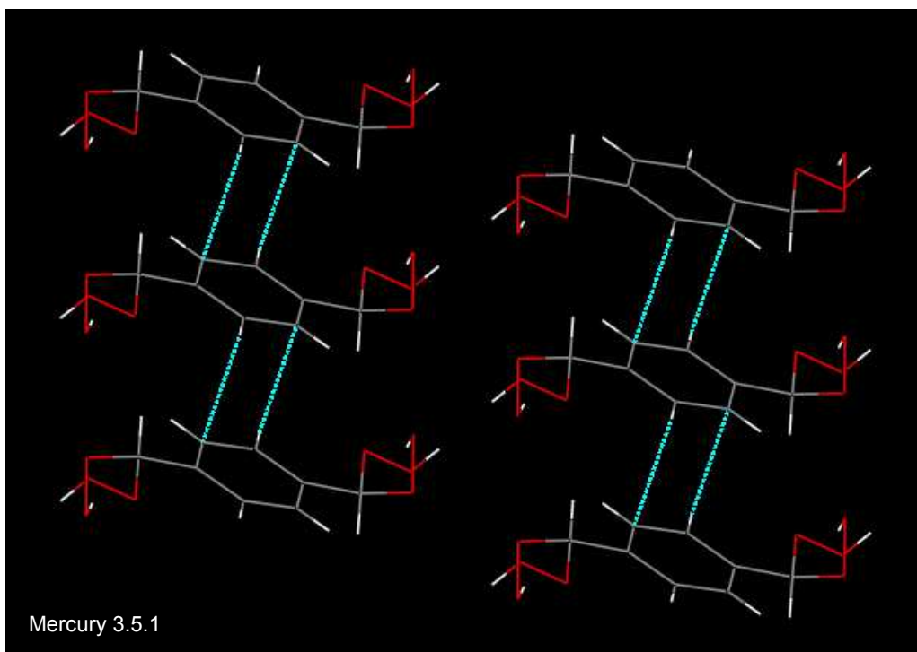
Figure 47. C-H... \pi interactions (blue) of 36 .
